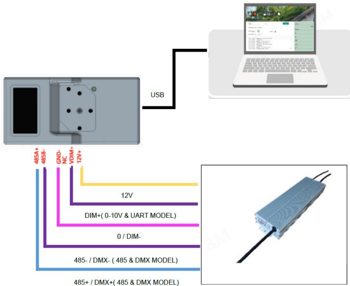
Figure 11. Programming Wiring
