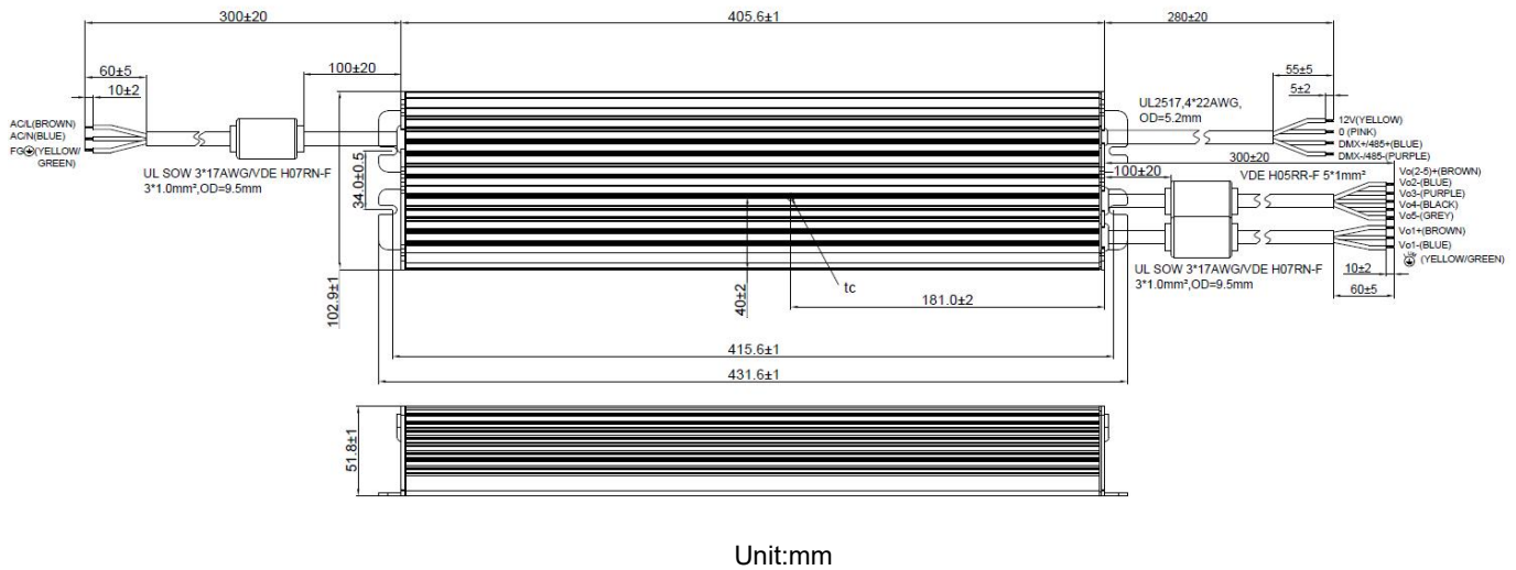
Figure 12. Mechanical Drawing
